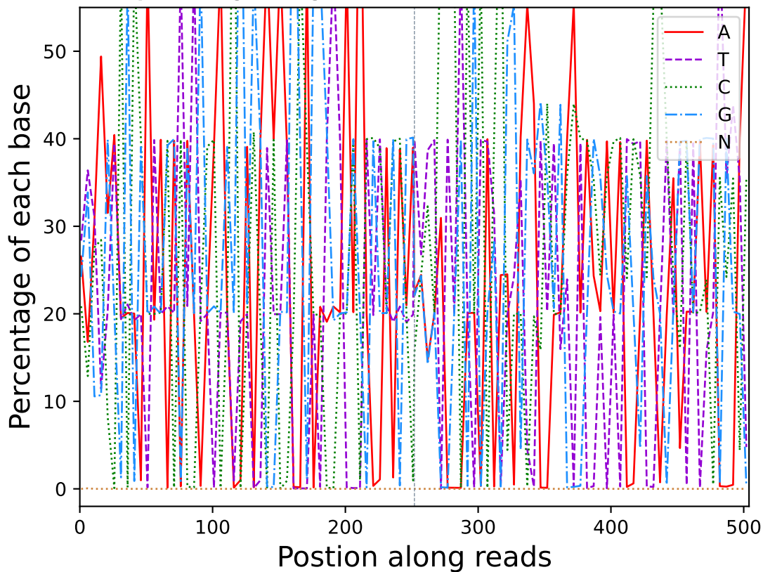
Base percentage along reads (R10516)
